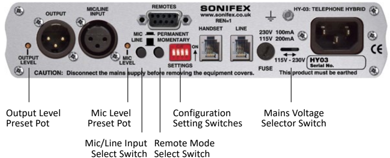
Figure 2-2 : Rear Panel Controls
